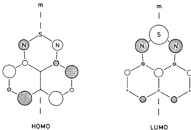
Fig. 5. Highest occupied and lowest unoccupied orbitals (HOMO and LUMO) of naphtho[1,8-cd]-[1,2,6]-thiadiazine ( 1 ). The areas of the circles are proportional to the squares of the LCAO coefficients. Blank and dotted areas symbolize opposite signs of these coefficients.
