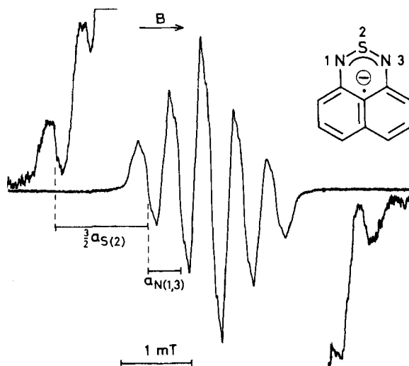
Fig. 4. ESR. spectrum of the radical anion of naphtho[1,8-cd]-[1,2,6]thiadiazine (1) showing the outermost ^{33}\text{S} -hyperfine components. Solvent DME, counter-ion \text{K}^+ , temperature 253 K.
